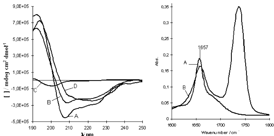
Figure 4. Left: CD spectra of (A) 21-mer 1 , (B) 14-mer 31 , (C) 7-mer 30 in TFE, as well as (D) 1 in egg yolk lecithin (80:1 w/w lipid/peptide) ( 5 \times 10^{-5} M) in MOPS 10 mM, 20% TFE pH 7.4. Right: FTIR spectra of 1 in TFE (A), and in lecithin vesicles (B).
