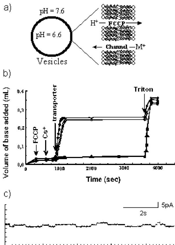
Figure 5. (a) Schematic generalization of the pH-stat method. The transport ability of test compounds is monitored by the release of protons from the vesicles as a function of time. (b) Illustrative example of results obtained using the pH stat technique. Cs + transport ability of monomeric crown ether 17 ( \Delta ), heptapeptide 30 ( \blacksquare ), hexacrown peptide 1 ( \bullet ), and Gramicidin A ( \circ ) (reprinted with permission of ACS). 29 (c) Single-channel conductance recordings of peptide 1 in 1 M KCl (at -100 mV, filtered at 200 Hz) in a DPPC bilayer (current level 3.5 \pm 0.2 pA, average lifetimes of open states > 1 s (reprinted with permission of Wiley-VCH)). 27
