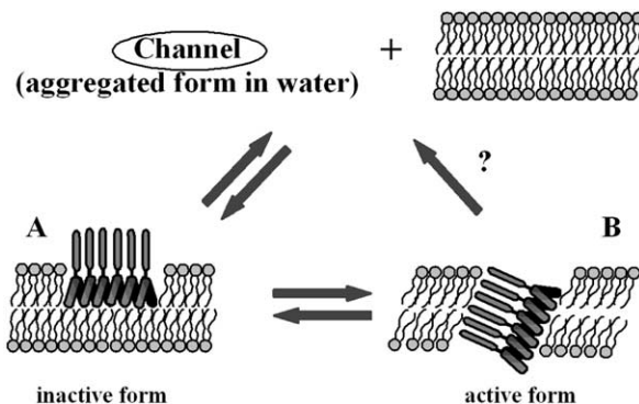
Figure 7. Proposed mode of action for the channel activity of peptide 1 . From the aggregates formed in the bulk water solution, one crown peptide adsorbs at the bilayer surface (A) and is in the adsorbed inactive form. From this partially incorporated form, peptide reorients itself into the active form B (reprinted with permission of Wiley-Interscience). 28
