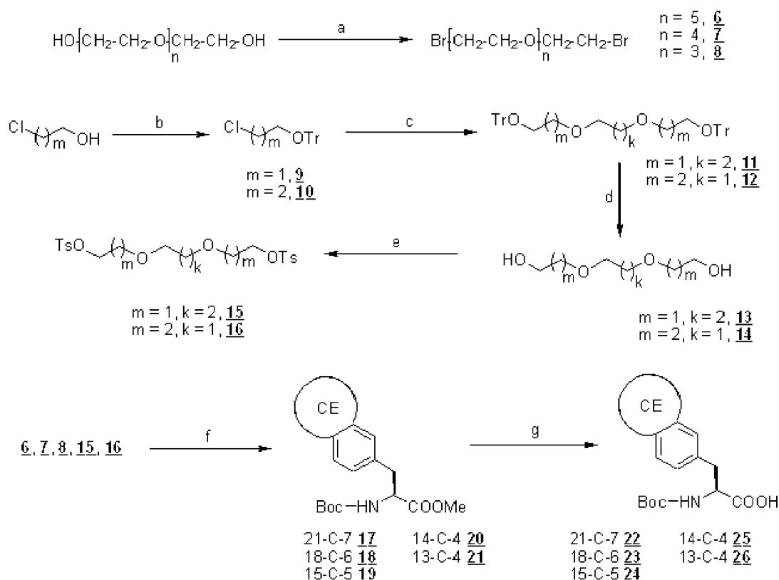
Figure 2. Synthesis of N - t -BOC protected crown ether amino acids: (a) \text{PPh}_3 , \text{Br}_2 , \text{CH}_3\text{CN} ; (b) \text{Et}_3\text{N} , \text{TrCl} , \text{DMAP} , \text{CH}_2\text{Cl}_2 ; (c) \text{NaH} , \text{HO}-(\text{CH}_2)_k\text{OH} ( k = 1, 2 ), \text{DMF} ; (d) 6\text{ N HCl/dioxane} , \text{CH}_2\text{Cl}_2 ; (e) \text{TsCl} , \text{Py} ; (f) \text{BOC-L-DOPA-OMe} , \text{Cs}_2\text{CO}_3 , \text{DMF} ; (g) 1\text{ N NaOH/MeOH} (CE, crown ether ring).
