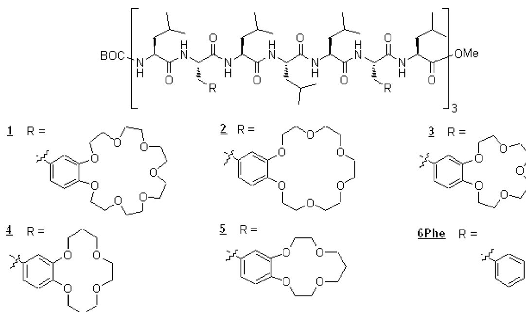
Figure 1. Crown peptide nanostructures synthesized and used in the present studies.
