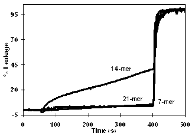
Figure 6. Calcein leakage induced by addition of 7-mer 30 , 14-mer 31 , and 21-mer 1 (5 mM) to phosphatidylglycerol/phosphatidylcholine (1:1) vesicles in HEPES 100 mM, NaCl 170 mM, EDTA 5 mM at pH 7.4. Vesicles were lysed with Triton X-100 at 400 s.
