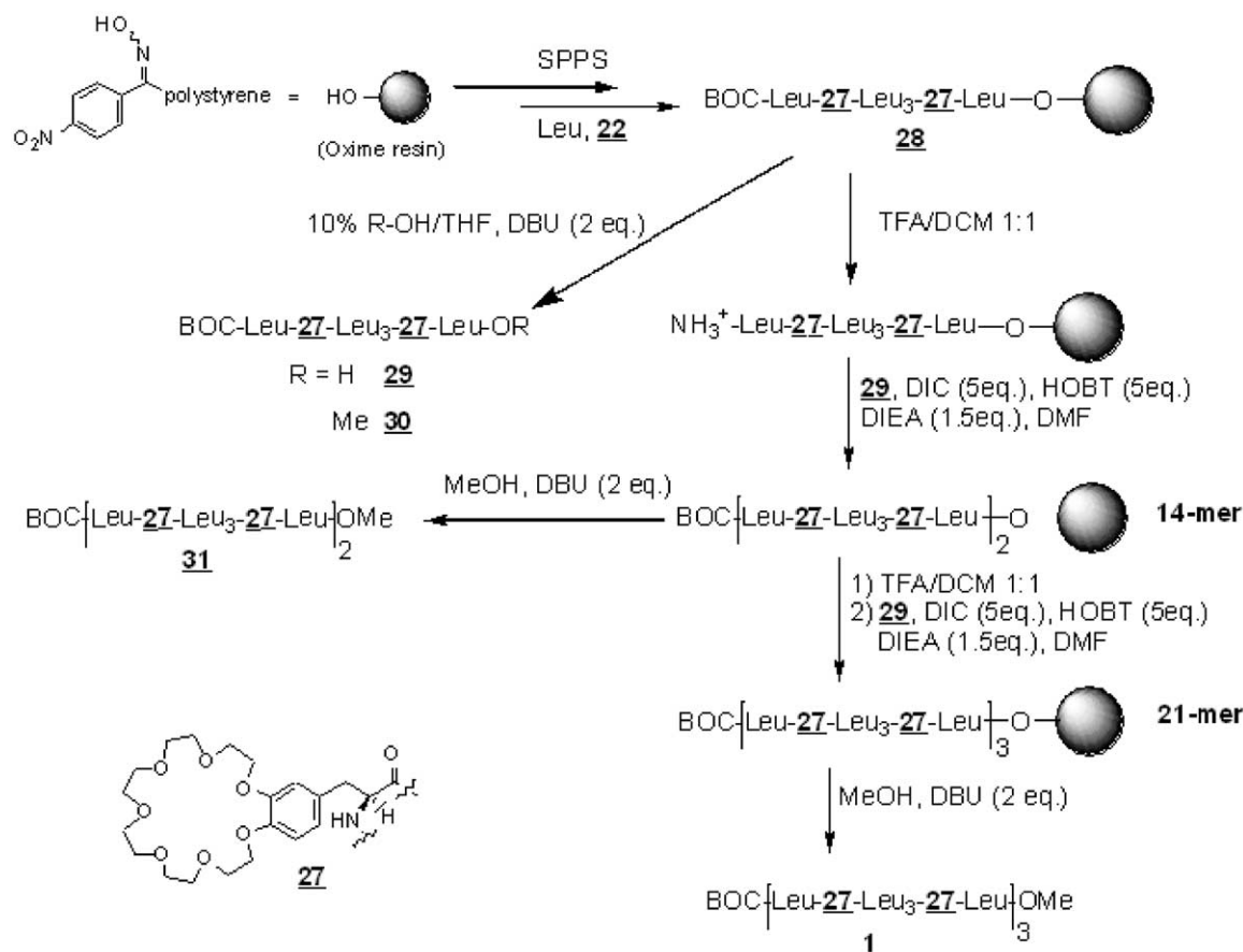
Figure 3. General synthetic strategy for the preparation of crown peptide nanostructures on oxime resin illustrated by the synthesis of the hexacrown peptide 1 .
